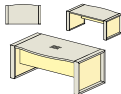
81S002 1800x1025x753
